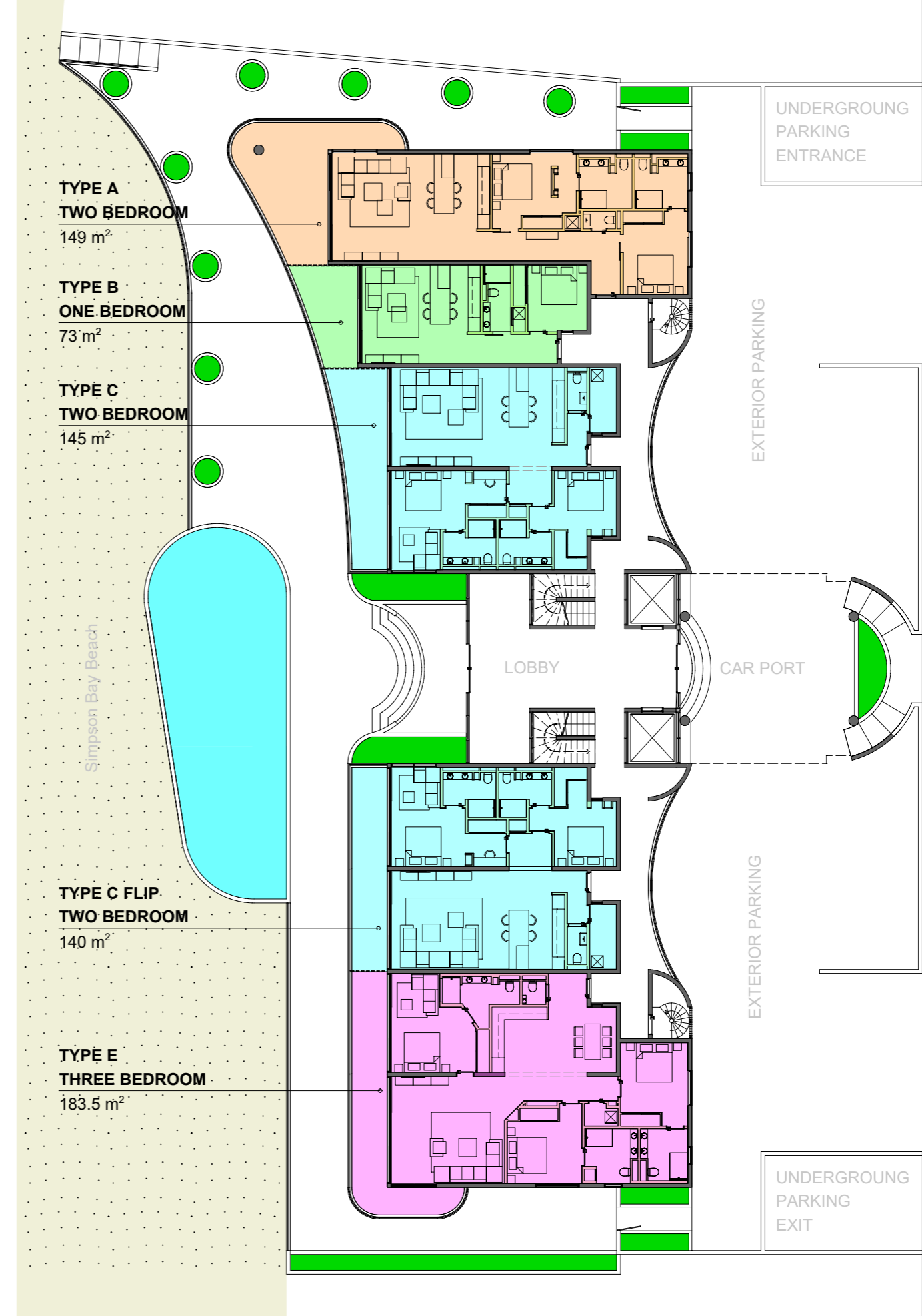
ALTERNATIVE FLOOR PLAN WITH 2 BEDROOM APARTMENTS (TYPE C)
